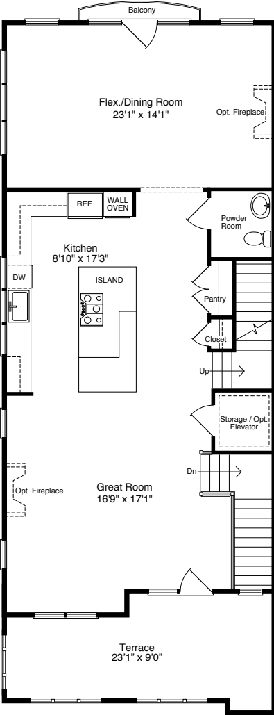
Second Floor Plan End Unit Window Patterns Vary By Elevation
